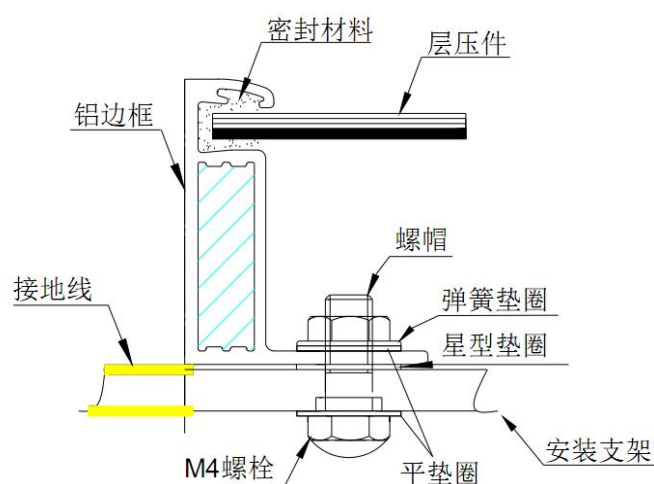
Figure 10-1 Grounding diagram
